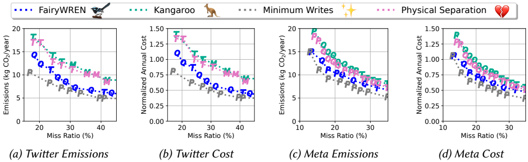
Fig. 13. The emissions and cost over six years for Kangaroo (🦘), FairyWREN (🧚), Min. Writes (🌟), and Physical Sep. (💔).
