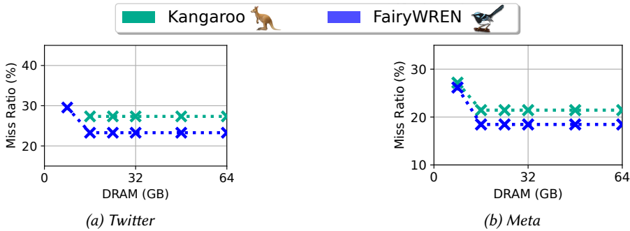
Fig. 20. Pareto curve of cache miss ratio at different DRAM sizes. The flash capacity is limited to 3.6TB, the desired lifetime is 6 years, and the caches use TLC flash.
