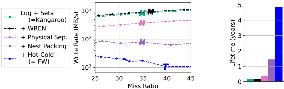
Fig. 18. Write rate (log-scale) and lifetime breakdown on the Twitter trace, incrementally adding optimizations to go from Kangaroo to FairyWREN.
