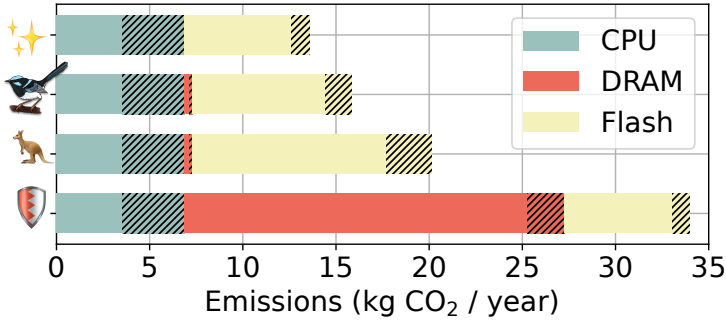
Fig. 13. Yearly carbon emissions for 4 caching systems: minimum writes (✦) with a write amplification of 1 with no additional DRAM, FairyWREN (🦉), Kangaroo (🦘), and a Flashfield-like log-structured cache (🛡️). Our results include the embodied and operational (hatched) emissions from CPU, DRAM, and flash.
