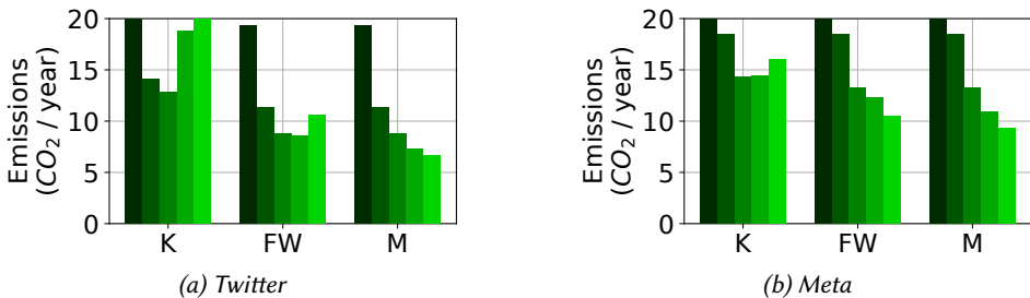
Fig. 14. The carbon emissions to achieve a 30% miss ratio on Twitter trace or 20% miss ratio on Meta trace on different flash densities for a desired lifetime of 6 years. Each bar for each cache represents a different density from SLC (left, darkest) to PLC (right, lightest).
