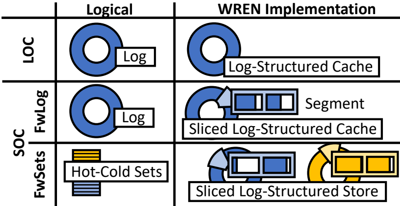
Fig. 7. The components of FairyWREN.
