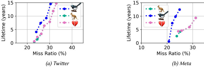
Fig. 17. The lifetimes for a 3.6 TB cache for Kangaroo (🦘), FairyWREN (🐦), and Physical Separation (❤️).
