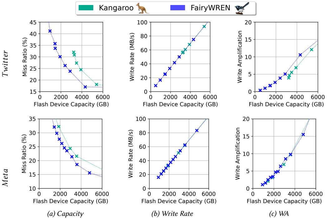
Fig. 19. Pareto curve of cache miss ratio at different flash device sizes and the corresponding write rate and write amplification of these points. The DRAM capacity is limited to 32 GB, the desired lifetime is 6 years, and the caches use TLC flash.
