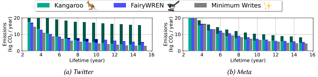
Fig. 15. The carbon emissions to achieve a 30% miss ratio on Twitter trace or 20% miss ratio on Meta trace with different lifetimes on QLC flash. The darker part of each bar represents emissions due to overprovisioning.
