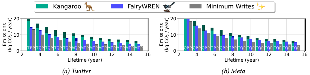
Fig. 16. The lowest carbon emissions to achieve a 30% miss ratio on Twitter trace or 20% miss ratio on Meta trace while varying both desired lifetimes and flash density. The darker part of each bar represents emissions due to overprovisioning. Letters on each bar represent the flash density
